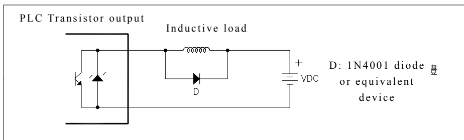
Suppress by a diode (for low power)
