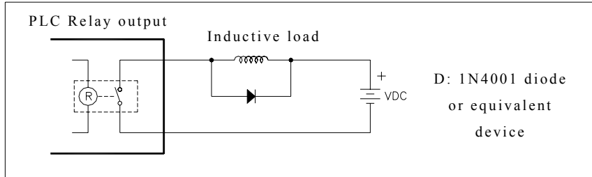
Suppress by a diode in DC power load (for low power)
