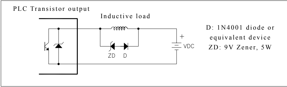
Suppress by a diode + Zener (high power and frequent ON/OFF)
