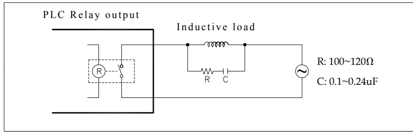
Scheme of AC power load
